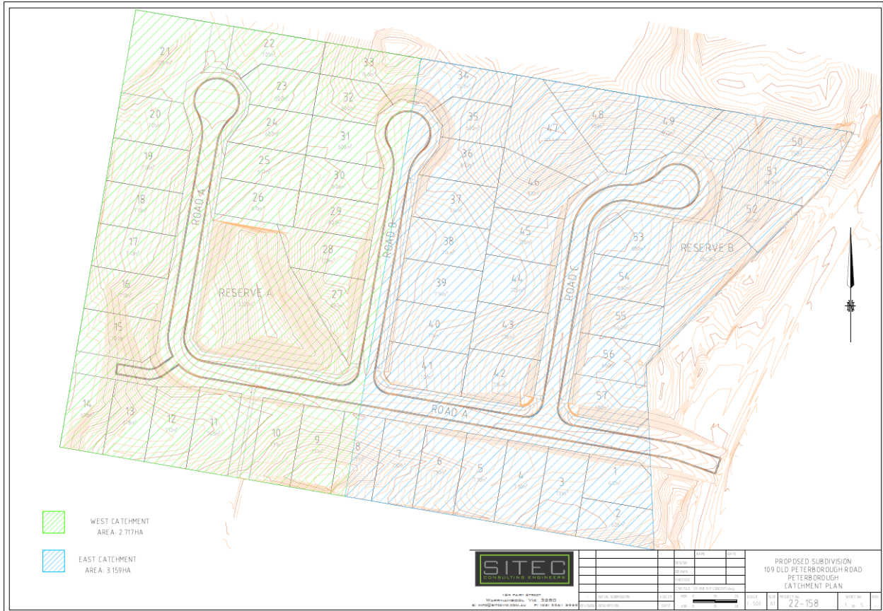
Figure 5 – Site subdivision catchment plan (Source: SITEC 2024).
